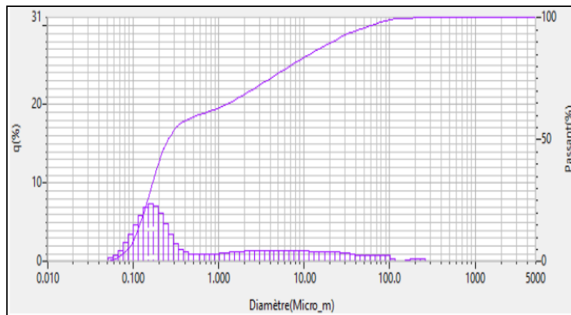
Figure 3. Particles size distribution of the powder
