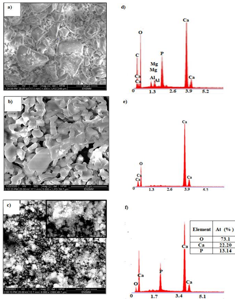
Figure 6. SEM /EDX of the HA synthesize a) MEB Eggshell powder, b) MEB Calcined eggshell powder, c) MEB Powder synthesized, d) EDX Eggshell powder, e) EDX Calcined eggshell powder, f) EDX Powder synthesized
