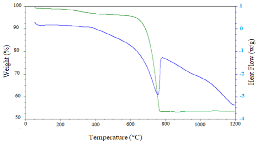
Figure 2. Differential thermal analysis of raw eggshell
