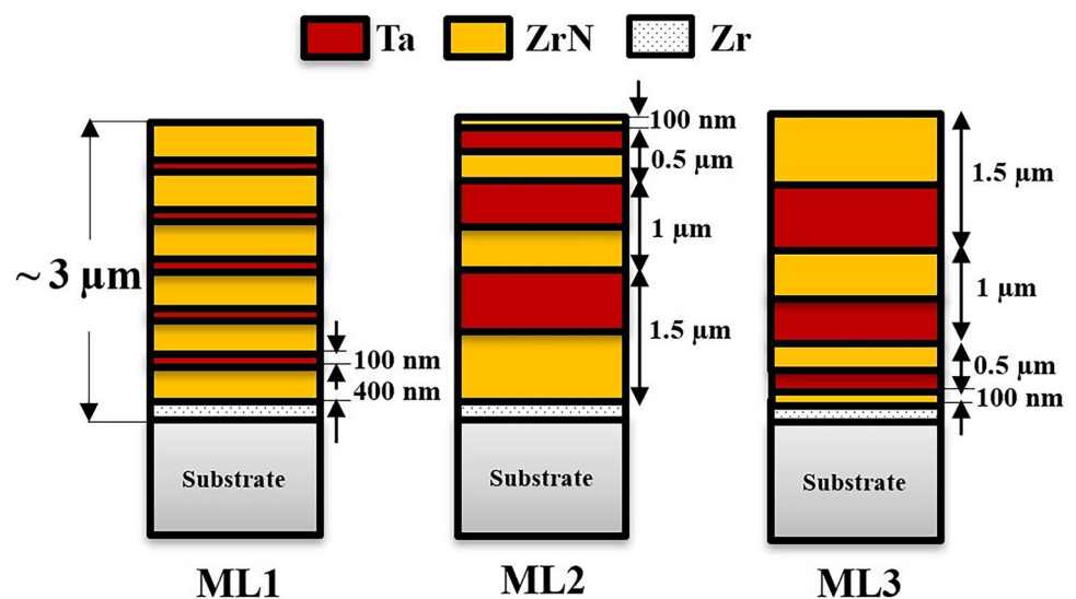
Fig. 1 Scheme of the architecture of the deposited (Ta/ZrN) multilayer coatings
