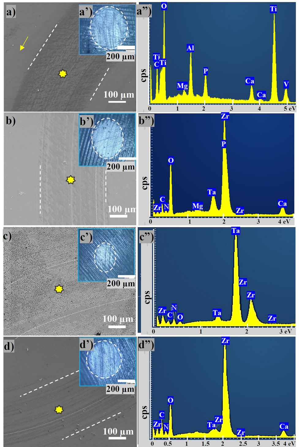
Fig. 7 SEM images, EDS microanalysis of samples, and optical images of the UHM-WPE ball after ball-on-disk testing for (a–a'') uncoated, (b–b'') ML1 coated, (c–c'') ML2 coated, and (d–d'') ML3 coated Ti-6Al-4 V disks
