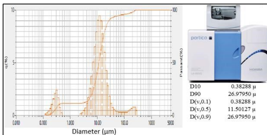
Figure 9. Particle size analysis of SHA calcined at a temperature of 850 °C prepared by co-precipitation
