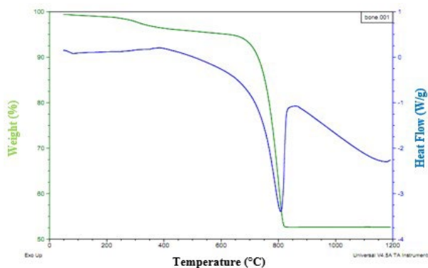
Figure 3. Differential thermal analysis of raw bone
