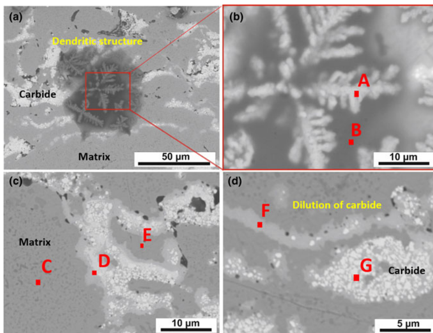
Figure 3: (a and b) Micrographs illustrating the dendritic structure in the binder matrix after annealing at 800 °C. (c and d) SEM cross-sectional micrograph of the dilution of carbide after annealing at 800 °C.
