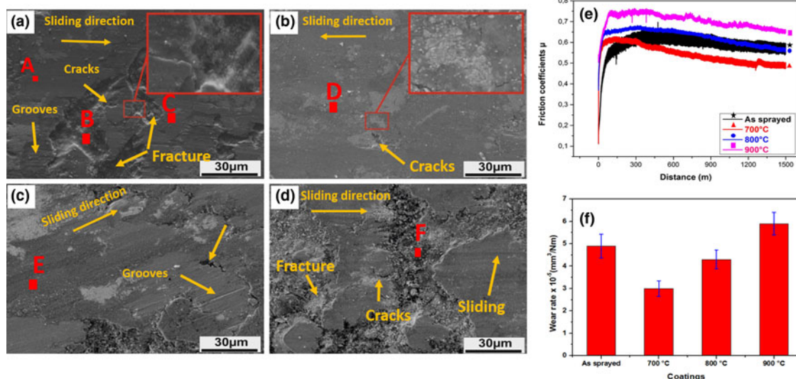
Figure 6: SEM micrograph showing the wear track of (a) as-sprayed and annealed coatings at (b) 700 °C, (c) 800 °C, and (d) 900 °C. (e) Friction coefficient data during tribotesting under a load of 15 N and a sliding distance of 1500 m. (f) Histogram showing the wear rate for pre- and post-annealed samples.
