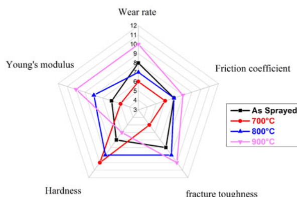
Figure 7: Polar diagrams providing a visualization of different results (hardness, Young's modulus, wear rate, friction coefficient, and fracture toughness) for the coatings investigated in this study.
